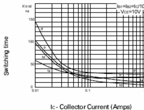
Switching Speeds
